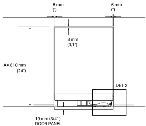
TOP VIEW EXTENDED INSTALLATION
