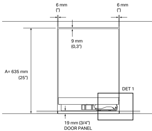
TOP VIEW FLUSH INSTALLATION
